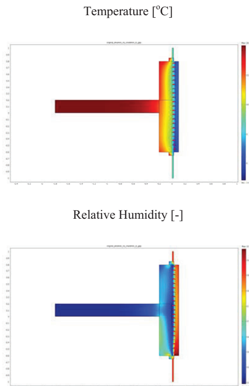
Figure 5 the original non insulated facade
