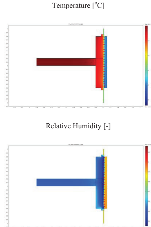
Figure 6 mineral wool in gap
