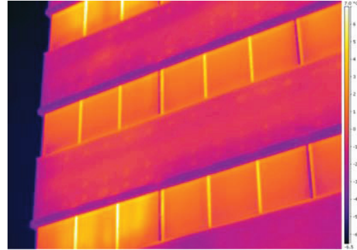
Figure 3 Infrared thermal image of the facade
