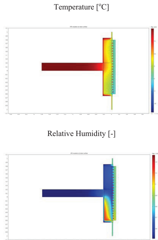
Figure 8 inside surface insulation with XPS
