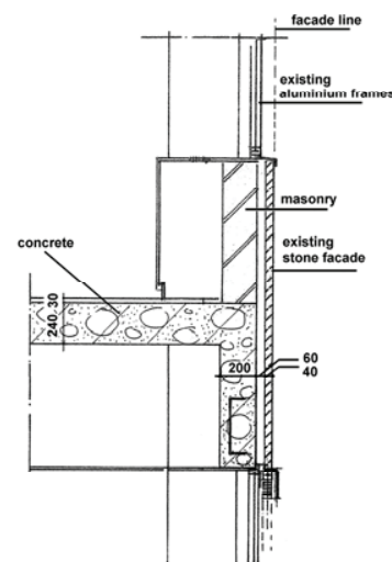
Figure 2 Vertical section of the facade
