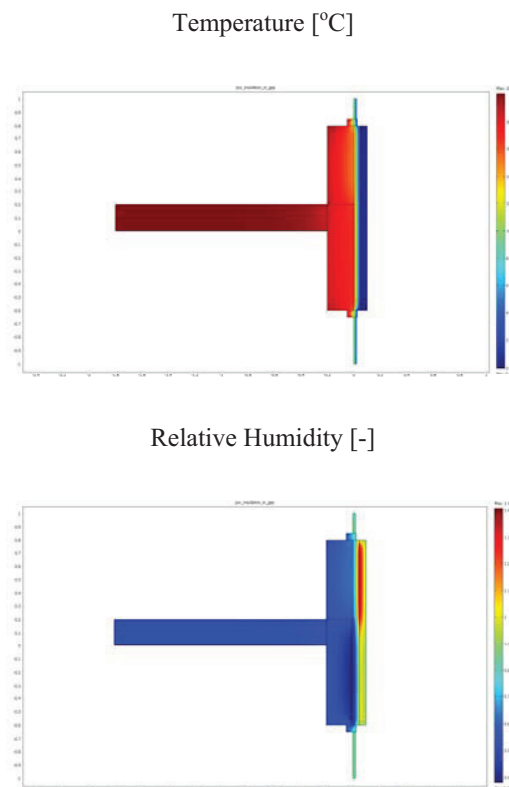
Figure 7 polyurethane in the cavity
