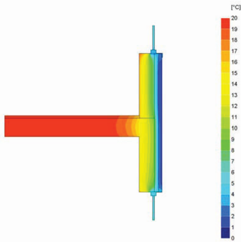
Figure 4 Thermal bridge calculations in BISCO of the insulated construction
